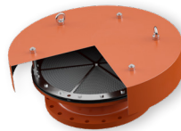
End-of-Line Deflagration Arresters EVA
